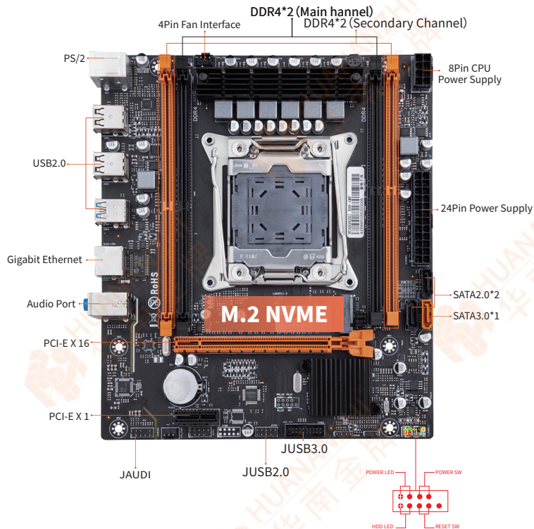
1-1 X79-4MF Motherboard illustration
